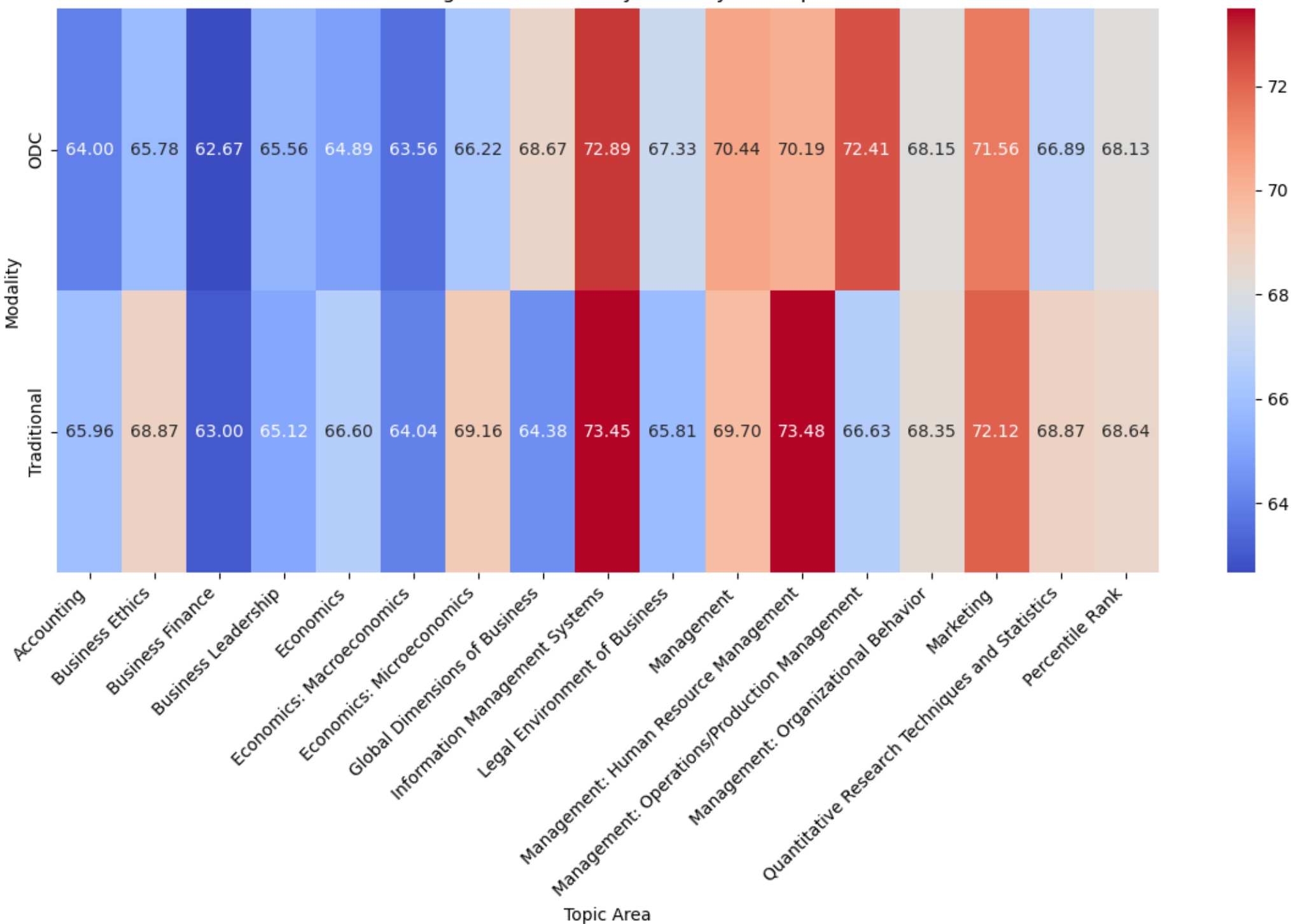
Average Performance by Modality and Topic
